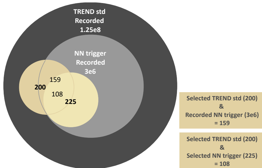
Figure 7: Diagram of coincidences that have been recorded (grey circles) and that have been selected (sand circles) with the TREND standard analysis (darker) and with our Neural Network trigger (lighter).
