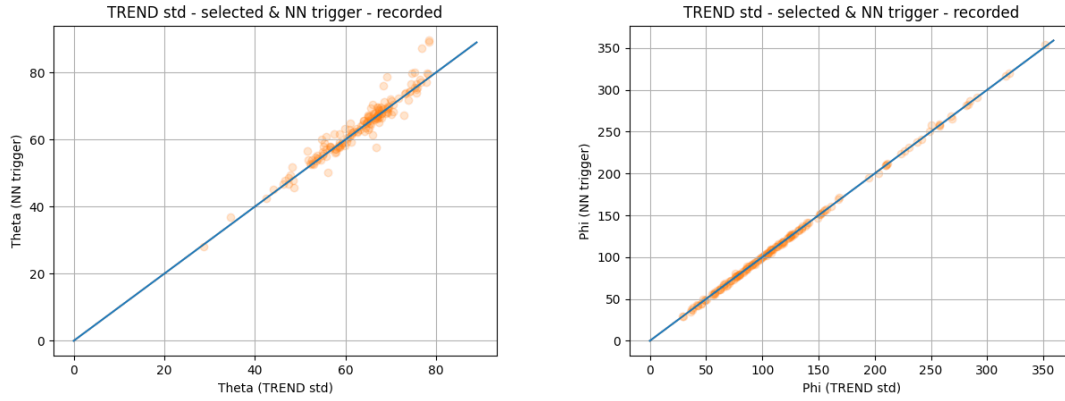
Figure 5: Zenith (left) and azimuth (right) angles for the 159 coincidences that were both selected by the TREND standard analysis and recorded by the Neural Network trigger. Angular reconstruction differs because of a loss of multiplicity due to the Neural Network veto on traces.
