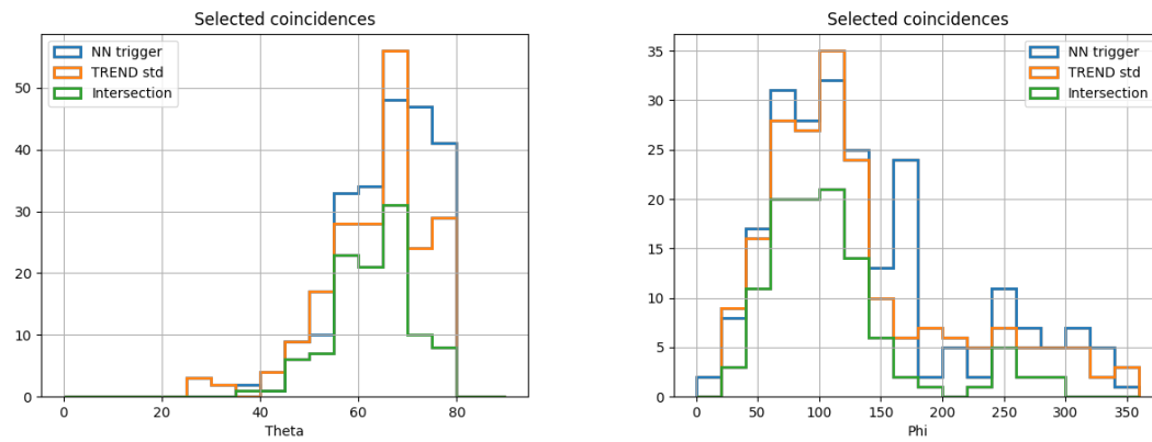
Figure 6: Zenith (left) and azimuth (right) distributions for selected coincidences (degrees). In blue with the Neural Network trigger and a set of offline cuts (225), in orange with the TREND standard trigger and selection (200). The intersection of the two selections is in green (108).
