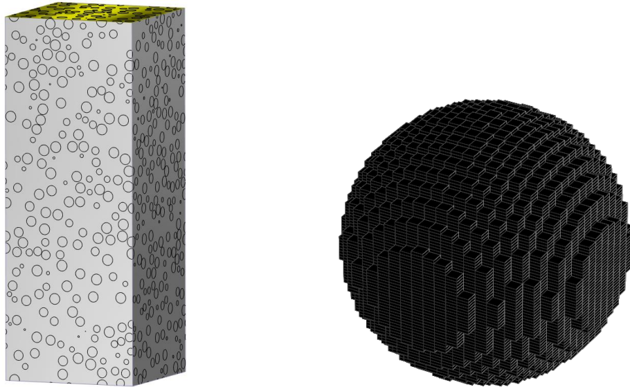
Configuration for 3D computation with 24% aggregates Aggregate description over the regular grid FIGURE 4. Configuration and aggregate description for 3D simulations
