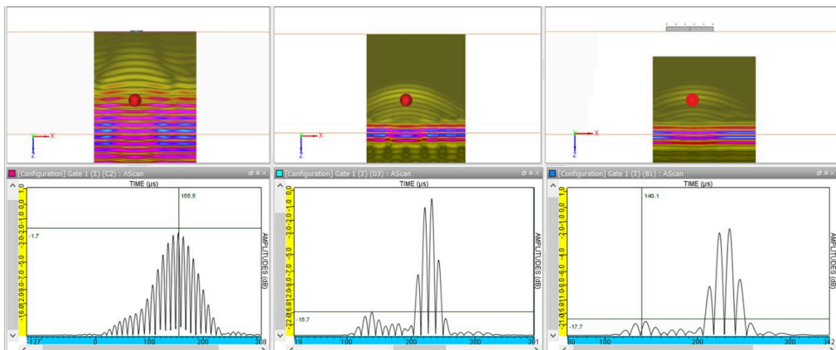
Figure 3: B-Scan images (at the top) and A-Scan signals when probe above defect location (at the bottom) for 3 ultrasonic transducers (from left to right: L0° probe, S1802, PL200 shear waves 0°)
