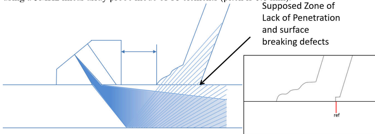
Figure 11: Inspection plan for RWS bridge deck
