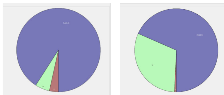
Figure 9: Sobol indices diagrams showing the shared influence of defect radius (in purple), depth (in green) and distributions (brown) on the signal amplitude for PL200 (left) and S1802 probes (right).
