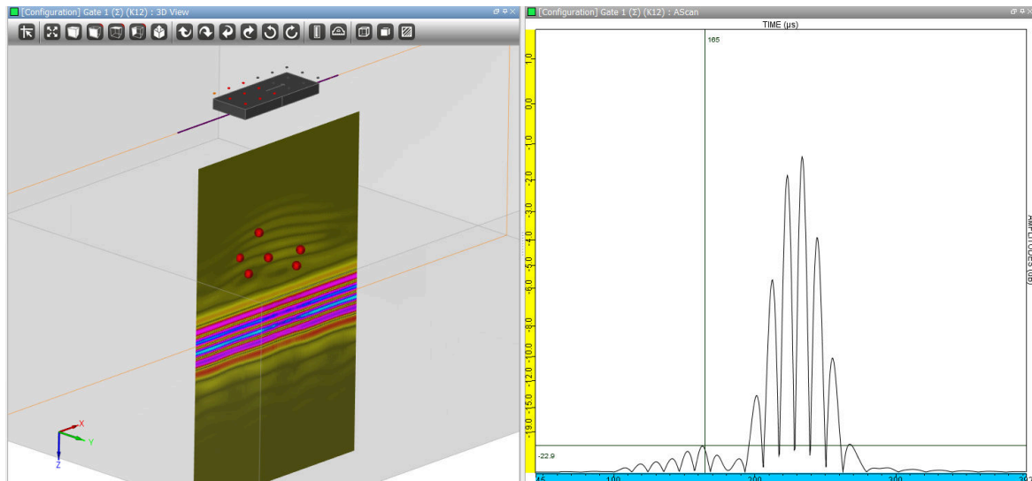
Figure 4: Model of a honeycomb defined by a set of 7 spherical flaws of 12 mm diameter each. Simulated B-scan (at the left) and A-Scan at the location of the max defect signal (at the right).
