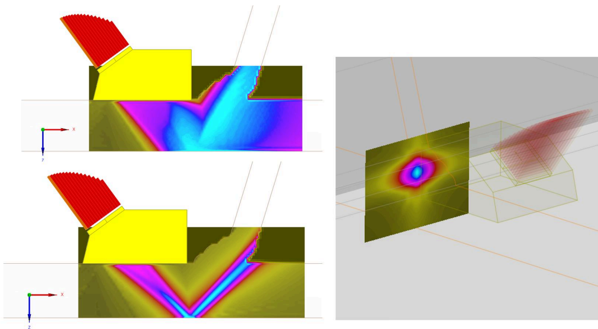
Figure 12: Beam coverage and beam spot characteristics
