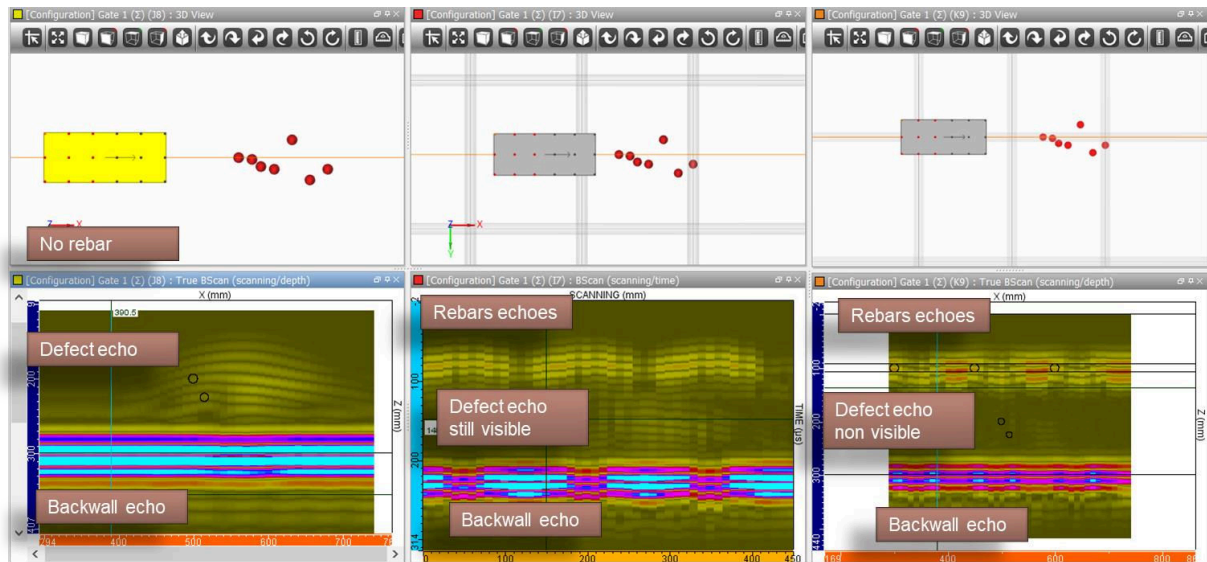
Figure 6: Simulations of defect responses without/with reinforcement steel bars.
