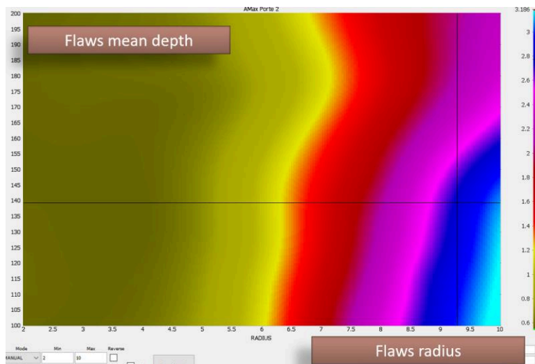
Figure 8: Joint influence of flaw size and depths variation on the signal amplitude observed on a 2D-plot obtained by metamodeling
