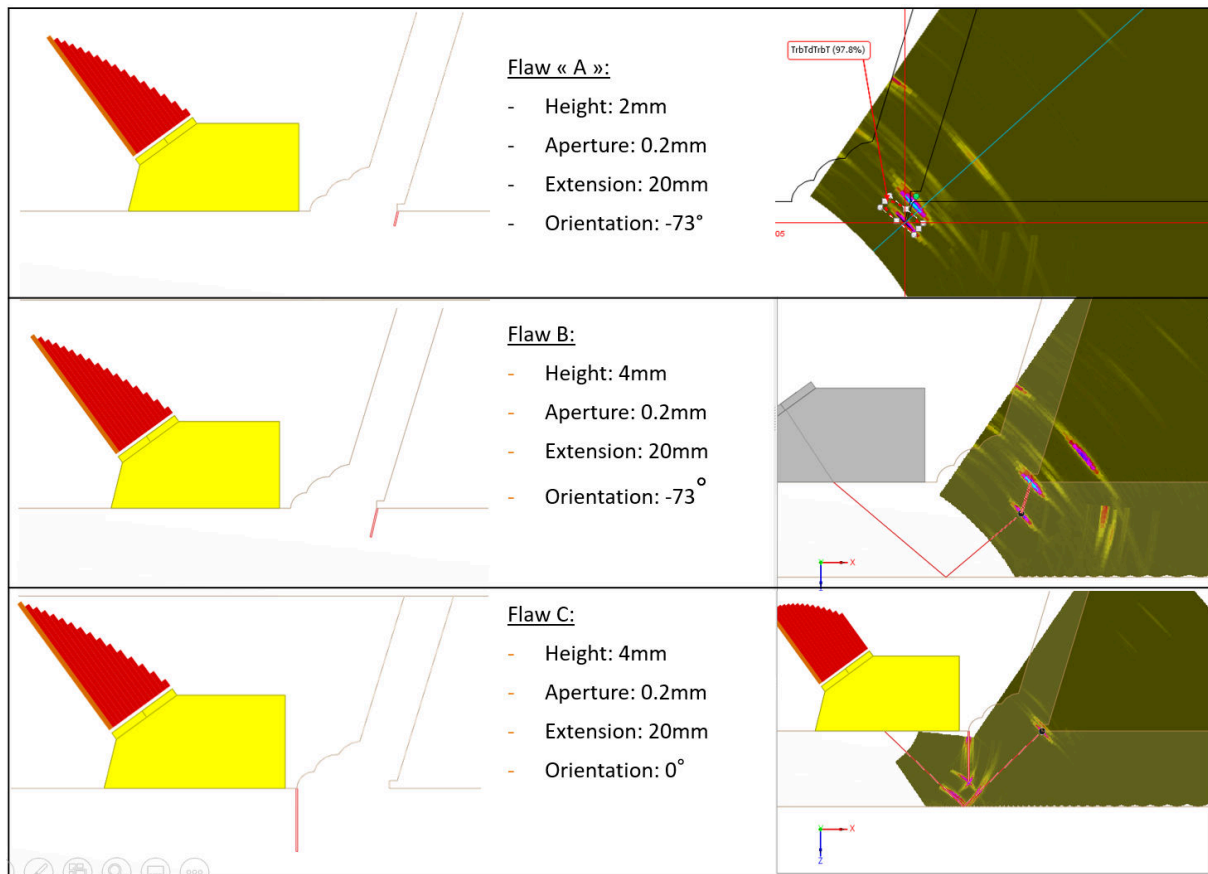
Figure 13: Simulated Defect scenarios and obtained sector scans
