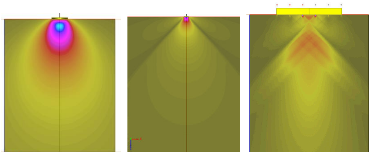
Figure 2: Ultrasound beam mapping for different probes (from left to right: L0° probe then S1802 and PL200 shear waves 0° probes)
