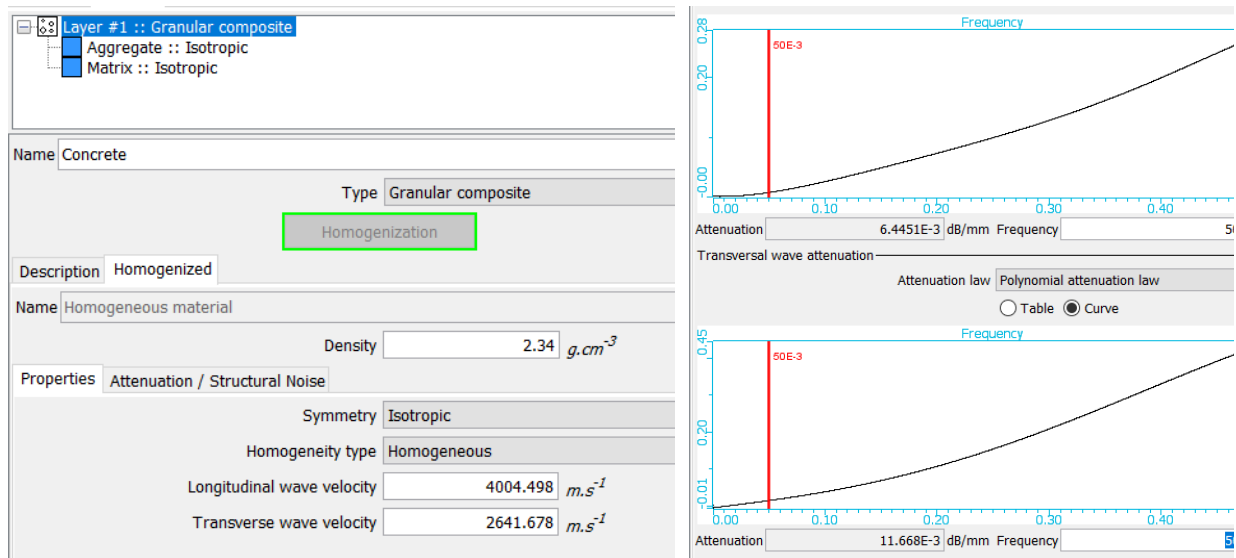
Figure 1: Concrete acoustic properties obtained after homogenizing initial input parameters
