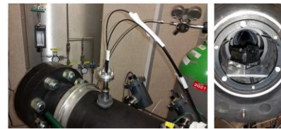
Fig. 5. View of the calibration experiment with the flame propagation tube (left), probe blocked inside the tube (right).
