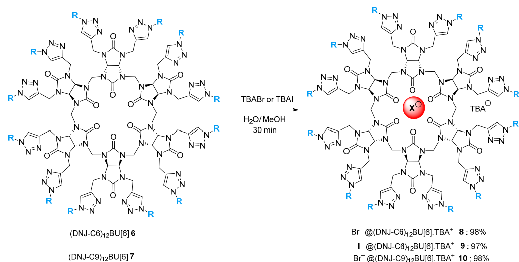
Scheme 4. Synthesis of \text{Br}^- @(\text{DNJ-C6})_{12}\text{BU}[6].\text{TBA}^+ 8 , \text{I}^- @(\text{DNJ-C6})_{12}\text{BU}[6].\text{TBA}^+ 9 and \text{Br}^- @(\text{DNJ-C9})_{12}\text{BU}[6].\text{TBA}^+ 10 .
