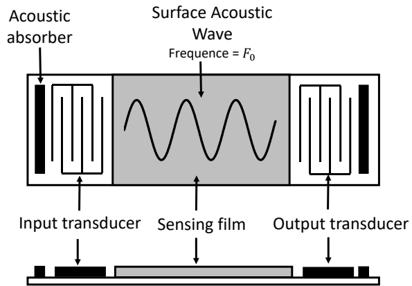
(a) The SAW sensor before any volatile chemical compound
