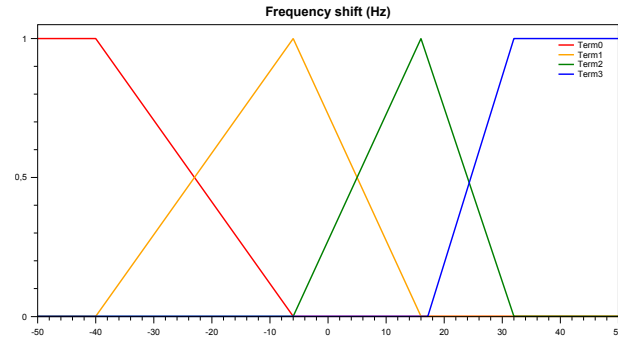
Fig. 4: Strong partition of the domain of an input variable, automatically obtained with a clustering approach
