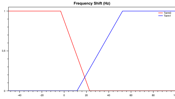
Fig. 3: Example of trapezoidal membership functions used in FURIA
