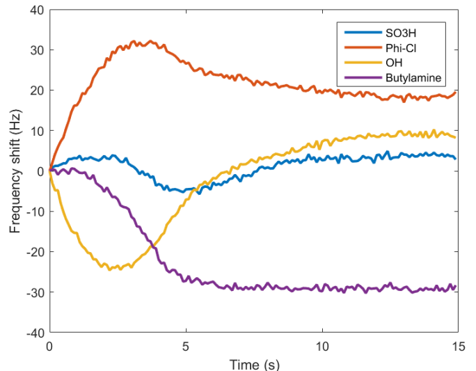
Fig. 2: Example of output of the sensor for a coffee capsule exposure.
