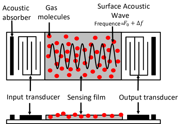
(b) The SAW sensor during an exposition to volatile chemical compounds
