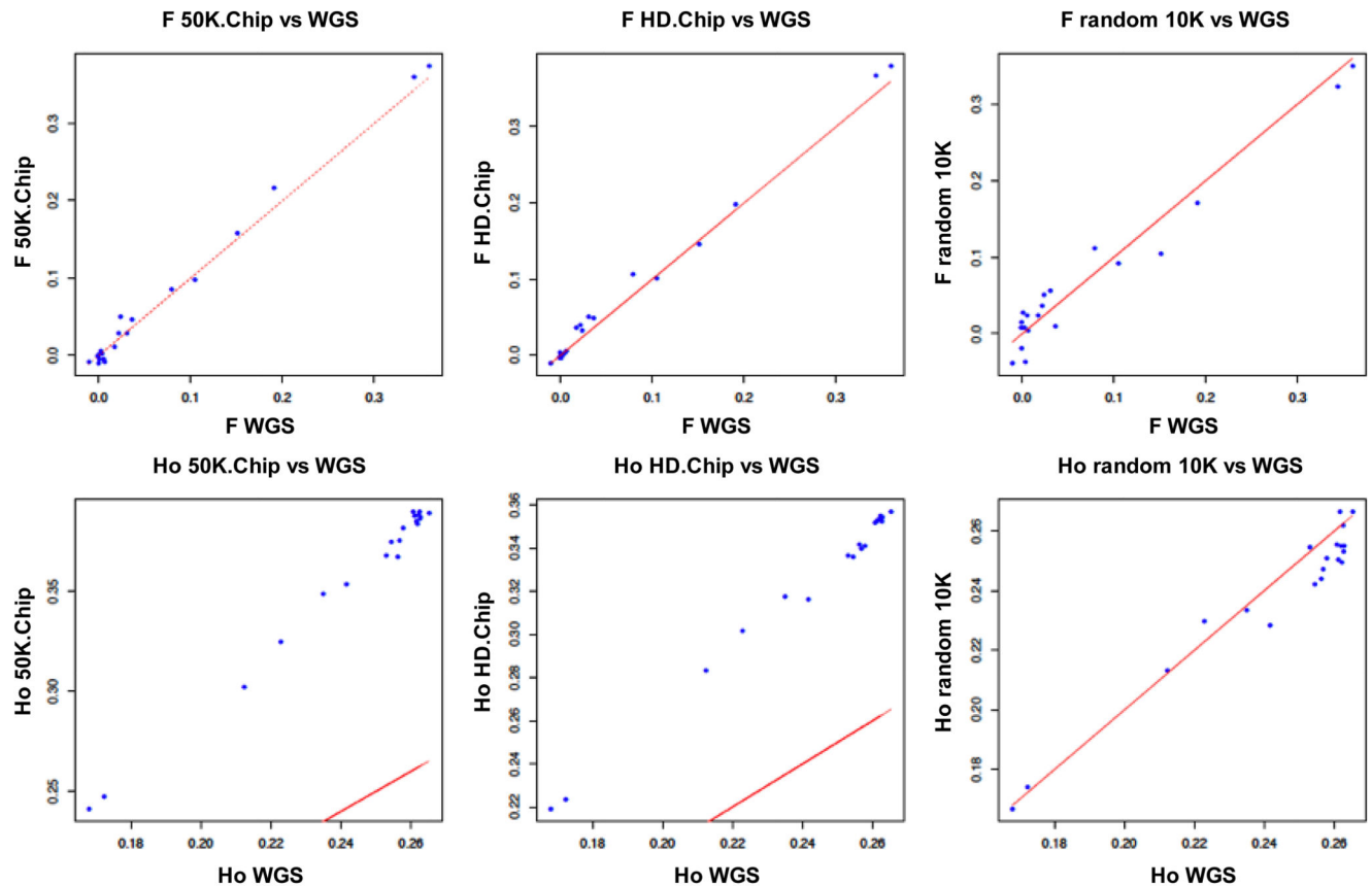
Figure 5. Estimates of individual inbreeding coefficient ( F ) and observed heterozygosity ( H_o ) from different panels of variants compared to WGS data estimates in sheep.
