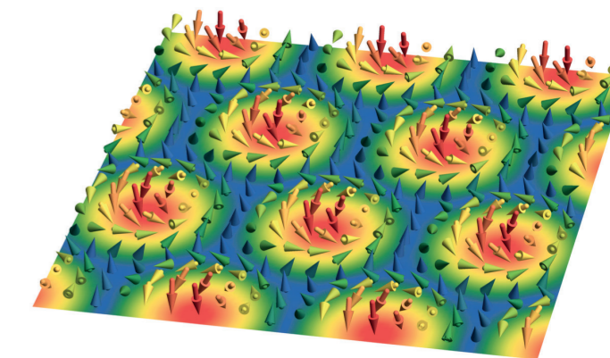
Nanometre-sized swirls of spins called Skyrmions are ideal candidates for spintronics and innovative data storage applications. © M. Garst - TU Dresden
