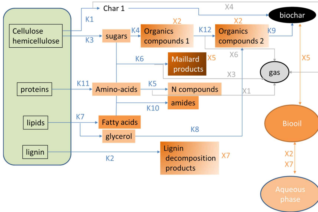
Figure 1 Global conversion mechanism for HTL of organic wastes
