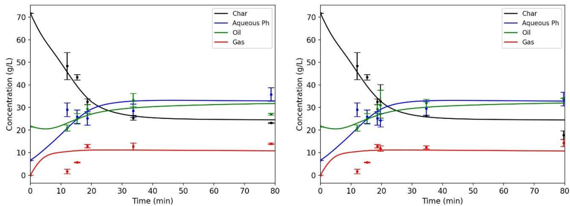
Figure 2 : HTL product yields for blackcurrant pomace at 300°C (left) and 315 °C (right)
