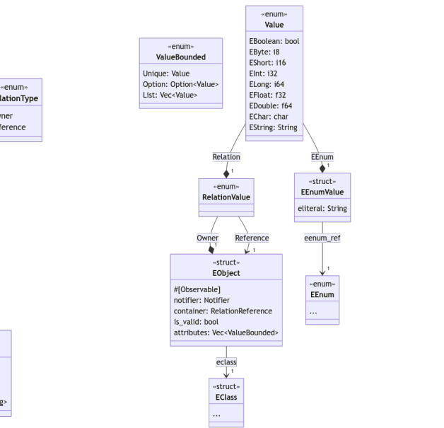
Fig. 4: Diagram of RustEcore for Creating Models
