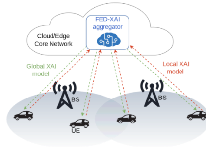
Fig. 2. FED-XAI approach.
