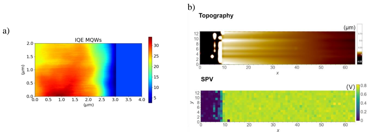
Figure 3: a) Internal quantum efficiency map (obtained from dividing the maps measured at room temperature and low temperature) and b) topography and SPV under maximum illumination maps ( 4 \times 0.8 \text{ μm}^2 , 64 \times 13 \text{ px}^2 ) on the border of a 1 \times 1 \text{ mm}^2 mesa.
