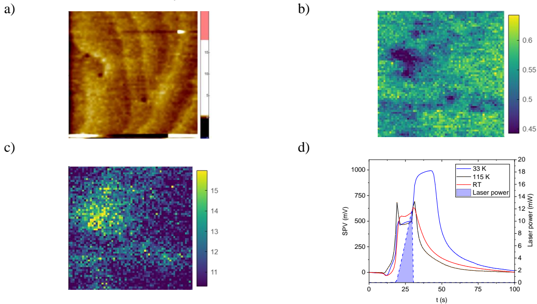
Figure 2: 800 \times 800 \text{ nm}^2 , 64 \times 64 \text{ px}^2 image on GaN-on-Si: a) topography (AFM) in nm, b) SPV at maximum illumination in mV, c) time decay constant map from the fit in each pixel in seconds and d) SPV vs. time as a function of laser power at three different temperatures.
