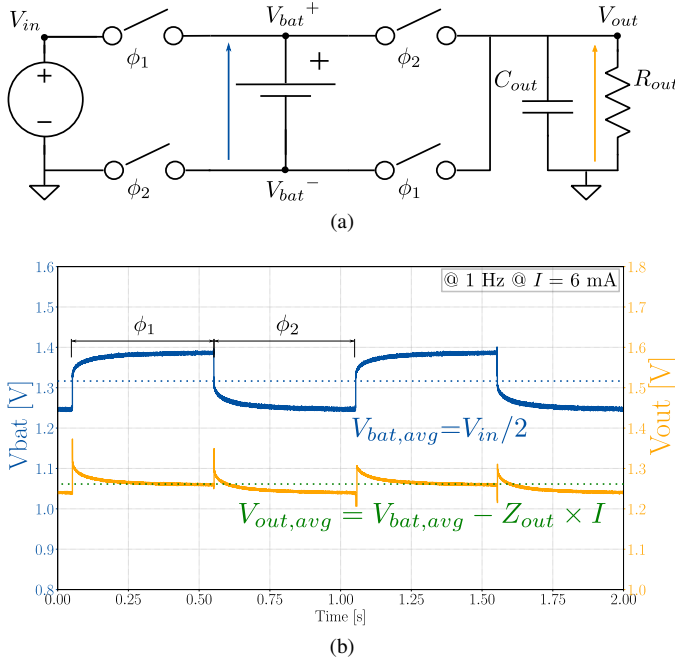
Fig. 4: (a) Electrical schematic of a 2:1 SBC and (b) Experimental voltage curves of battery and output in a SBC (without output capacitor) in steady-state
