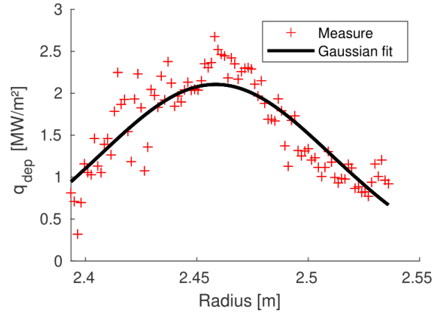
Figure 19. Power flux profile during pulse 55604 at t=5.78\text{s} .
