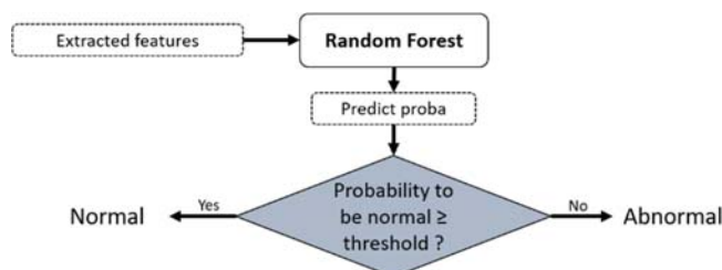
Fig. 4 Prediction block based on random forest classifier
