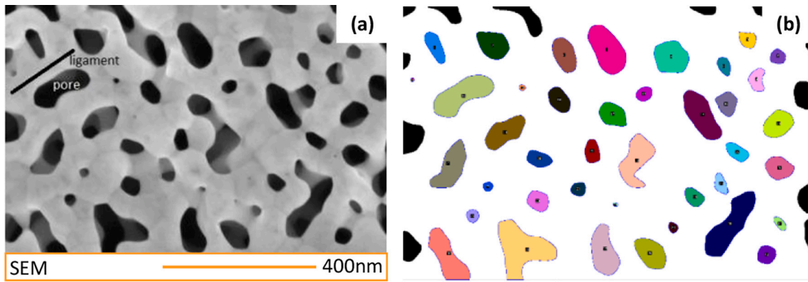
Fig. 4. Nanofoam after etching during 10 h with HNO 3 (17% dilution at 50 °C) (a)-SEM image (b)- ImageJ image processing.
