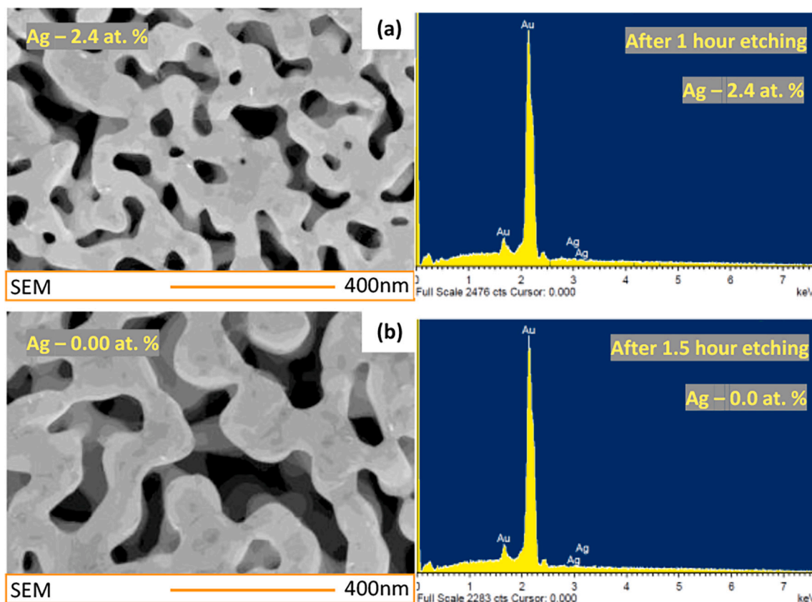
Fig. 7. Nanofoam fabrication: HNO 3 (50% dilution at 100 °C).
