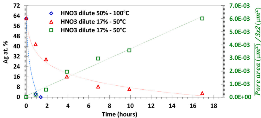
Fig. 8. Ag at.% and average pore area as a function of time etching for different temperatures and different HNO 3 concentrations.
