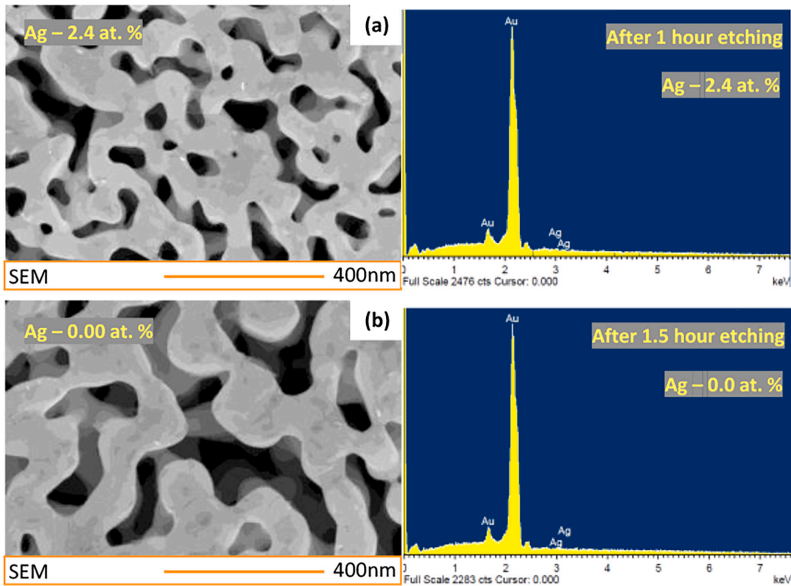
Fig. 7. Nanofoam fabrication: HNO 3 (50% dilution at 100 °C).
