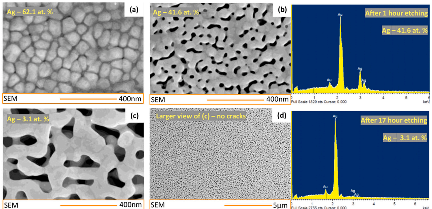
Fig. 6. Nanofoam fabrication: with HNO 3 (17% dilution at 50 °C).
