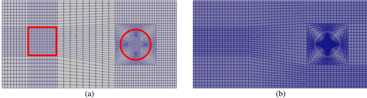
Figure 1: Example of mesh obtained for the benchmark by CIVAS SHM (a): macro-mesh with the delamination (red square) and transducer (red circle) and (b): spectral finite element mesh
