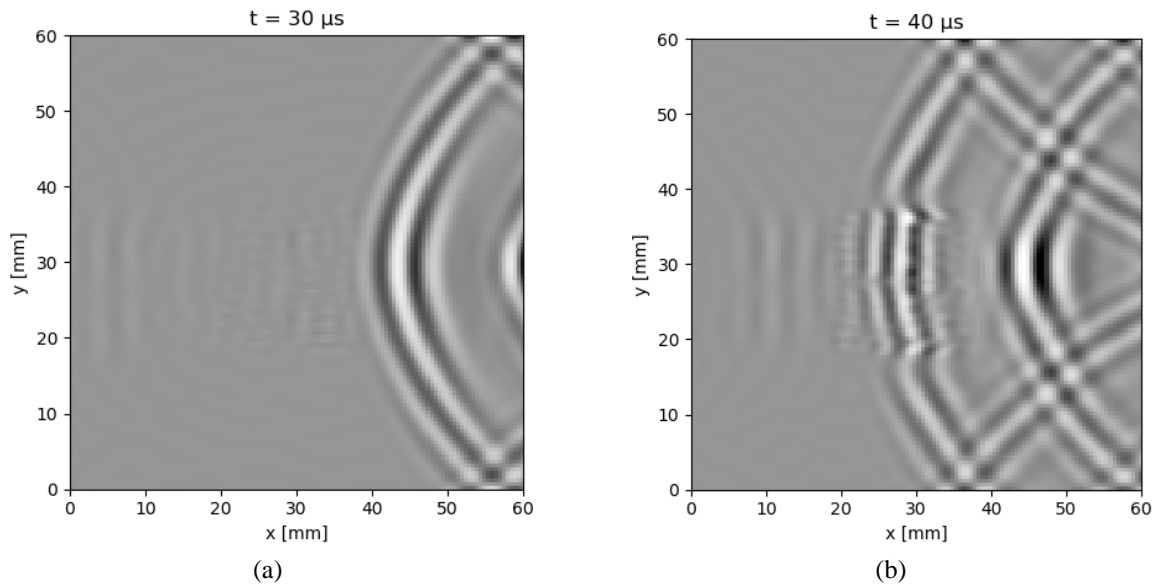
Figure 2: Snapshot of the out-of-plane wave velocity over the delaminated area (a): at 30\mu\text{s} and (b): and 40\mu\text{s}
