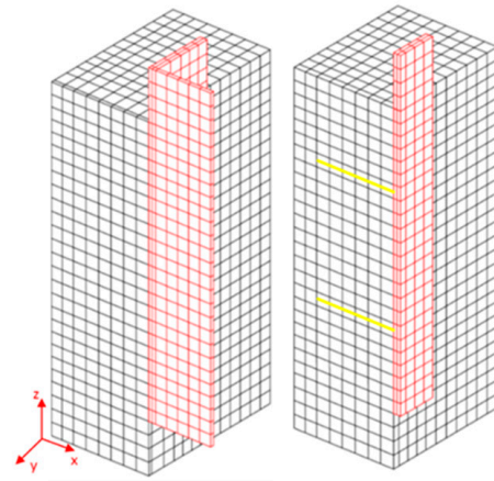
Figure 17. Mesh of a quarter of the ST25-A push-out test [42] modeled with the 1D simplified modeling (overall view and cross section at the stud level); concrete in black, steel beam in red, studs in yellow.
