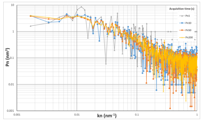
Fig. 13 : Power spectral density extract from the CD-SAXS measurements with different acquisition time. 1 second correspond to 2 acquisitions of 0.5s : 1 top position and 1 bottom position.
