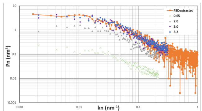
Fig. 15 : Power Spectral Density extracted from experiment (orange line) and the ones obtained from simulation with different value of roughness parameter \sigma , other roughness parameters \alpha and \xi have been respectively set to 0.463 and 26.36 nm
