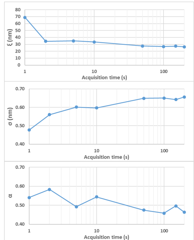
Fig. 14 : Extraction of roughness parameter from PSD fit as a function of diffraction acquisition time.
