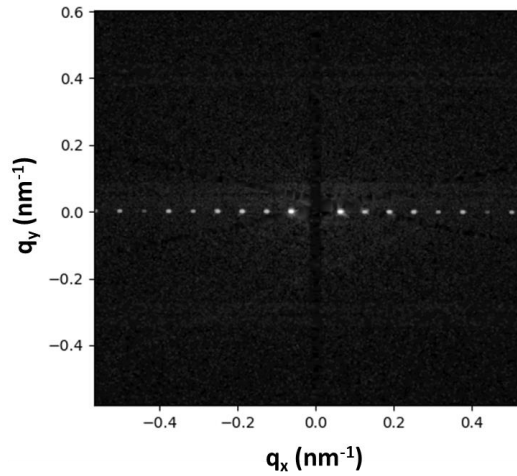
Fig. 5 : (q_x, q_y) reciprocal space map of the line gratings measure at \omega=0^\circ for sample "1-113-G".
