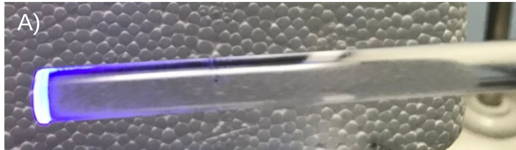
Scintillator E (Length : 0.6mm, Diam. : 6mm) PMMA wave guide (Length : 23cm, Diam. : 6mm)
