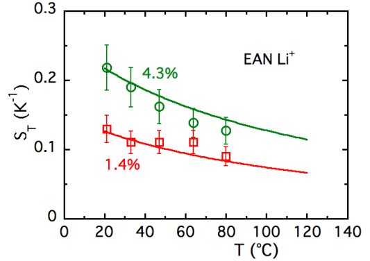
Fig. 6 Soret coefficient S_T as a function of T at different \Phi 's for the three counterions; The full lines correspond to the adjustments of S_T(T) with the formalism of Sections 3.2.4.
