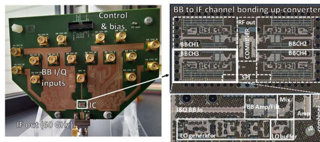
Fig. 2. BB to IF up converter board and IC photograph.
