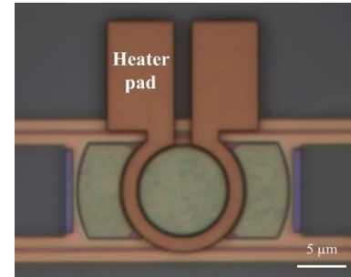
Figure 8. Optical microscope picture of Ti/TiN heater on top of MRR
