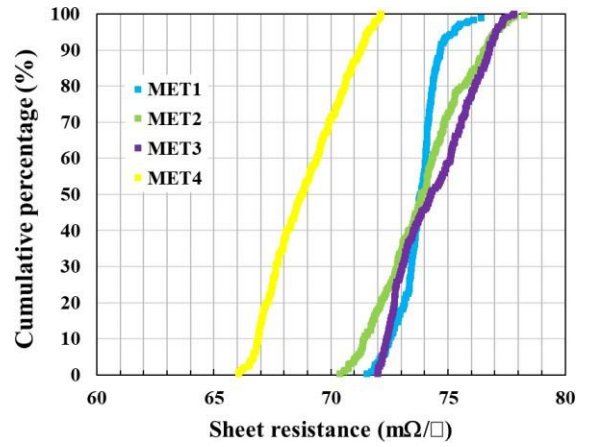
Figure 24. Back-end sheet resistance
