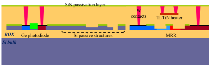
Figure 10. Schematic cross-section of the full PIC before TSV processing
