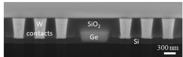
Figure 9. Germanium photodiode with W contacts
