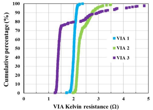
Figure 26. Back-end Via Kelvin resistance
