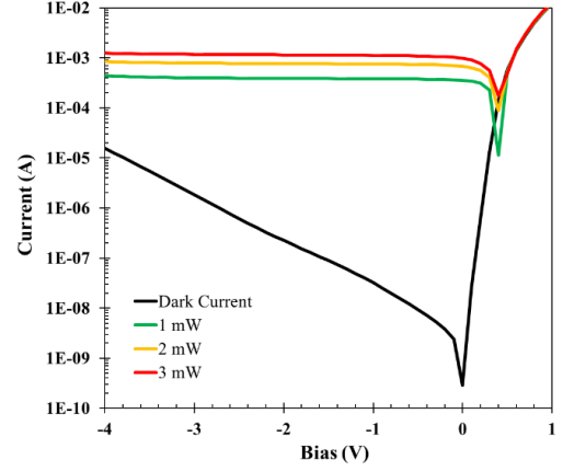
Figure 20. Dark current and photocurrent for various laser power vs voltage bias of 15 μm long photodiode with 1 μm intrinsic Ge width
