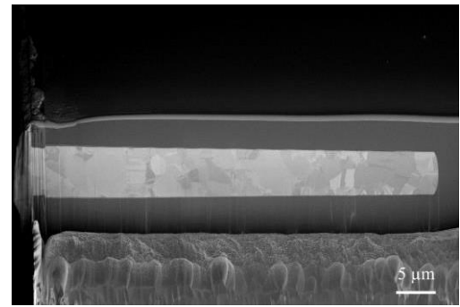
Figure 13. FIB/SEM cross-section of TSV middle after annealing
