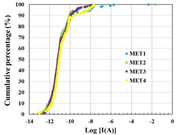
Figure 25. Back-end leakage current
