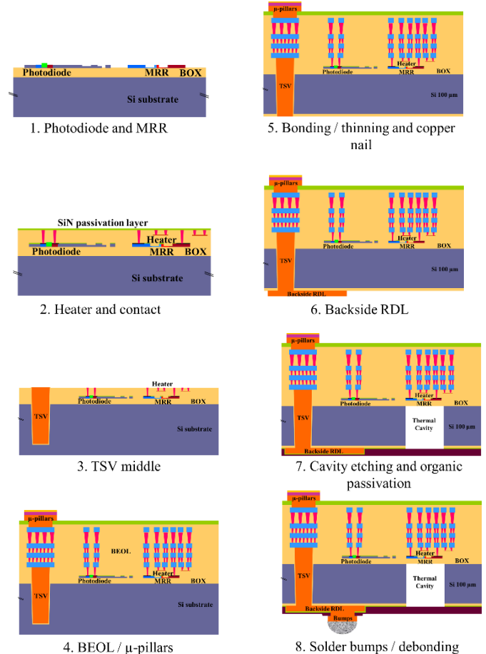
Figure 4. POPSTAR SiPho interposer schematic process flow
