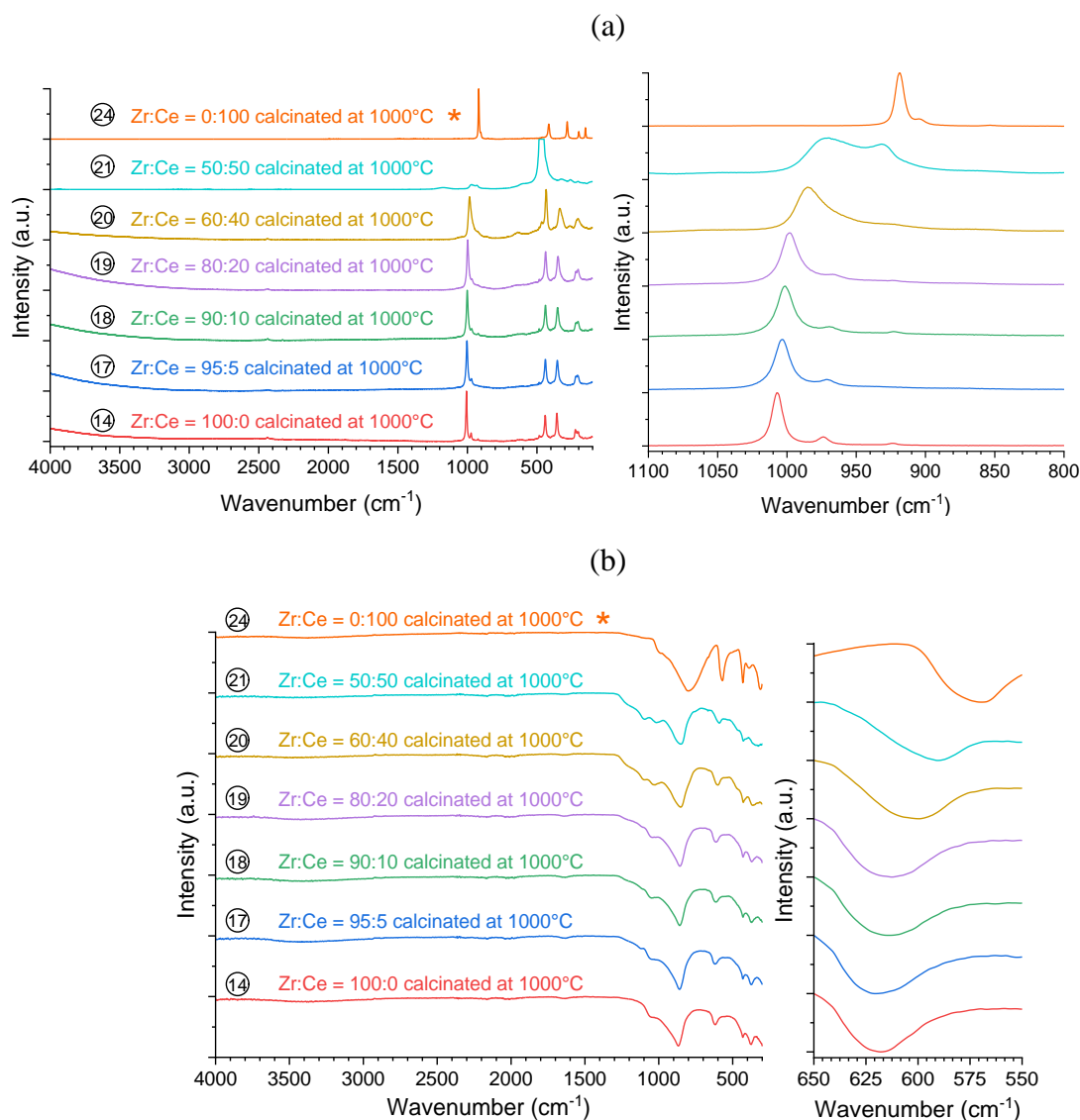
Figure 12. Raman (a) and IR (b) spectra recorded for annealed (\text{Zr,Ce})\text{SiO}_4 solid solutions with Zr:Ce = 100:0 (14), Zr:Ce = 95:5 (17), Zr:Ce = 90:10 (18), Zr:Ce = 80:20 (19), Zr:Ce = 60:40 (20), Zr:Ce = 50:50 (21) prepared under hydrothermal conditions ( T = 250^\circ\text{C} , 7 days, \text{pH} = 1.0 ) starting with Zr + Ce and silicate concentrations of 0.2 \text{ mol}\cdot\text{L}^{-1} . * Reference \text{CeSiO}_4 sample ( T = 150^\circ\text{C} , 7 days, \text{pH} = 6.5 ) starting with cerium and silicate concentrations of 0.2 \text{ mol}\cdot\text{L}^{-1} (24).
