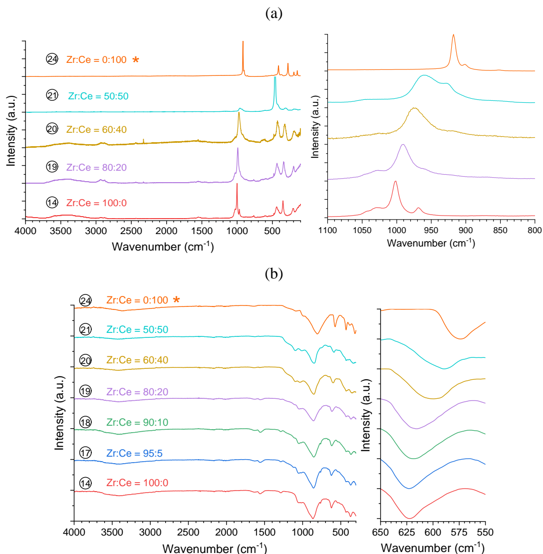
Figure 11. Raman (a) and IR (b) spectra recorded for pristine (\text{Zr,Ce})\text{SiO}_4 solid solutions with Zr:Ce = 100:0 (14), Zr:Ce = 95:5 (17), Zr:Ce = 90:10 (18), Zr:Ce = 80:20 (19), Zr:Ce = 60:40 (20), Zr:Ce = 50:50 (21) prepared under hydrothermal conditions ( T = 250^\circ\text{C} , 7 days, \text{pH} = 1.0 ) starting with Zr + Ce and silicate concentrations of 0.2 \text{ mol}\cdot\text{L}^{-1} . * Reference \text{CeSiO}_4 sample ( T = 150^\circ\text{C} , 7 days, \text{pH} = 6.5 ) starting with cerium and silicate concentrations of 0.2 \text{ mol}\cdot\text{L}^{-1} (24).
