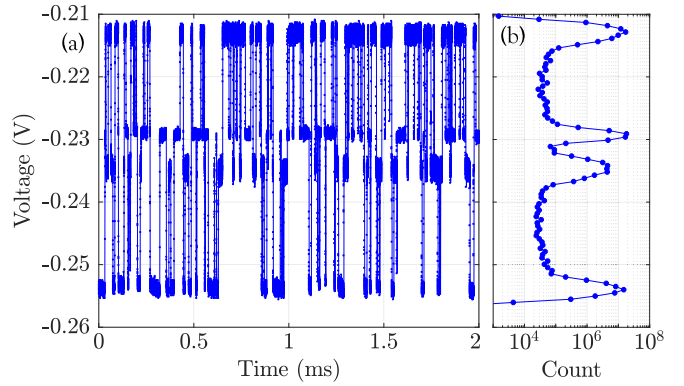
FIG. 3. (a) Time trace of the voltage of two coupled superparamagnetic tunnel junctions (SMTJs), for \mu_0 H = 6.9 mT, V_0 = -0.45 V, and R_0 = 473 \Omega . (b) Histogram of measured voltages over 20 s. Note the logarithmic scale on the horizontal axis.
