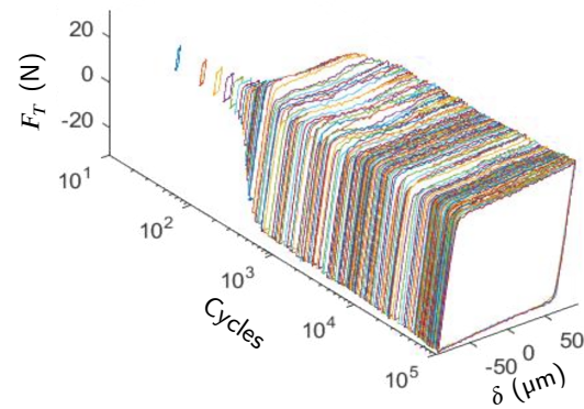
Figure 2: Fretting log for the wear test at P = 30 N, \delta = 80 \mu\text{m} for 100,000 cycles [26].
