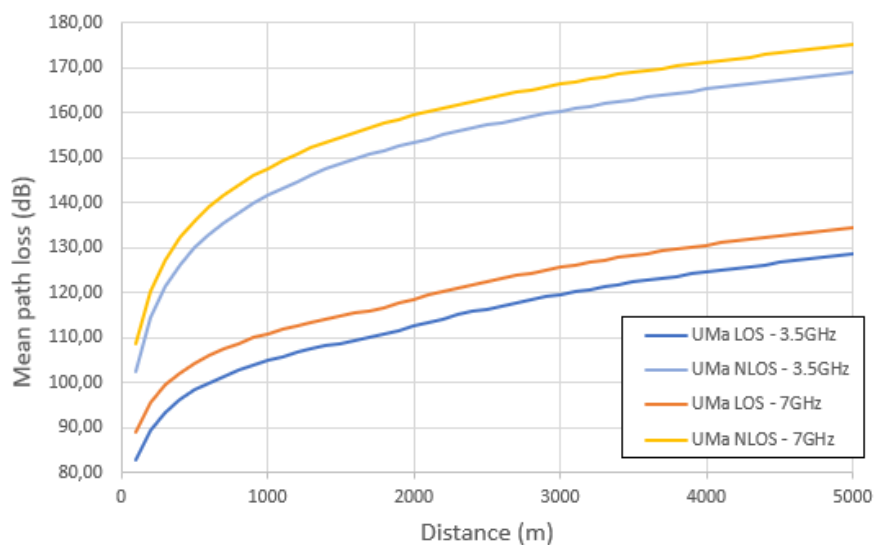
Figure 5 - Mean path-loss vs. distance from the 3GPP UMa model at frequencies 3.5 GHz and 7GHz.
