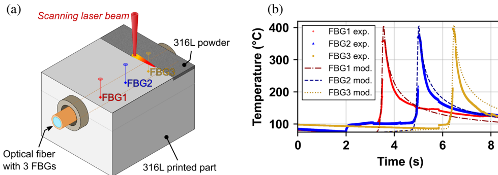
Fig. 1 (a) Schematic of L-PBF monitoring using an array of three FBGs (not to scale); (b) Comparison between experimental and simulated temperature values for each FBG sensor during the manufacturing of one layer.
