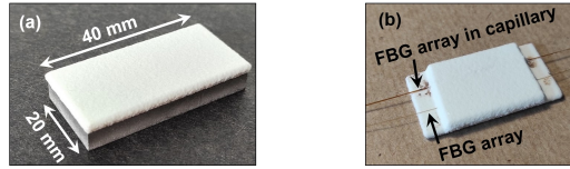
Fig. 1. (a) APS target for OFS embedding. (b) Embedded sensors in cordierite after the first thermal annealing.
