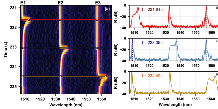
Fig. 3. (a) Reflected spectra amplitude as a function of time and wavelength for layer #11. (b)–(d) Spectra for maximum BWS of the different FBGs in the timespan. Vertical lines represent peak position calculated with the 3-dB BW algorithm.
