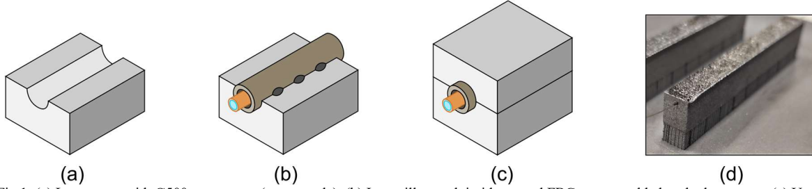
Fig 1. (a) Lower part with \varnothing 500\ \mu\text{m} groove (not to scale). (b) In-capillary polyimide-coated FBGs array welded to the lower part. (c) Upper part printing for sensor embedding. (d) Finished part after unmelted powder removal.
