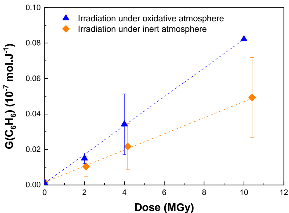
Figure 2. Evolution of G(\text{C}_6\text{H}_6) , the gaseous benzene emission radiation chemical yield (in \text{mol.J}^{-1} ) as a function of dose and the irradiation atmosphere.
