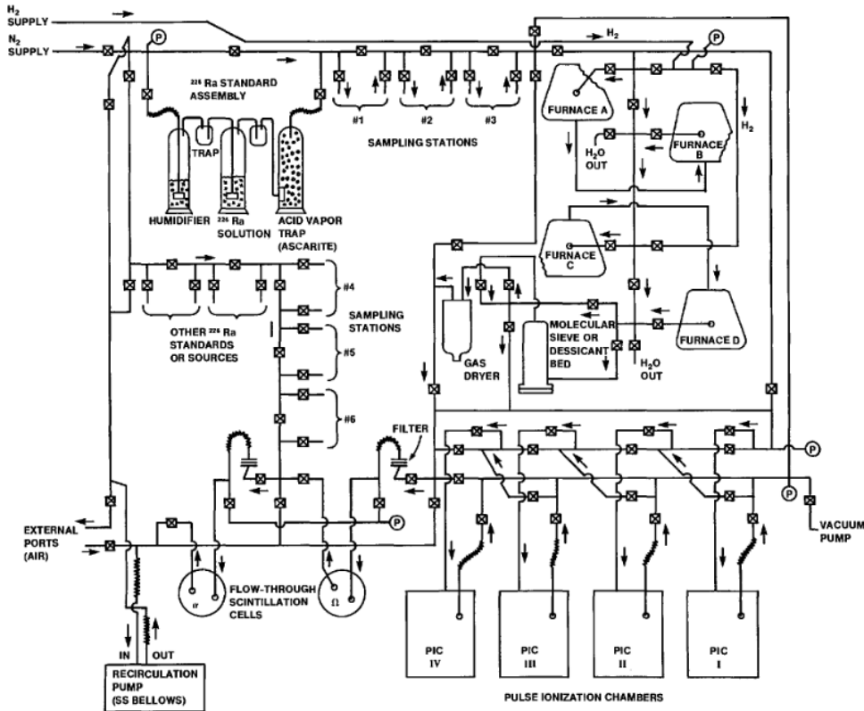
A simplified schematic of the NIST primary radon measurement system illustrating its major components and principle of operation. R Collé, et. al., The NIST primary Radon-222 measurement system (1990) J. Res. Natl. Inst. Stand. Technol. 95, 155
