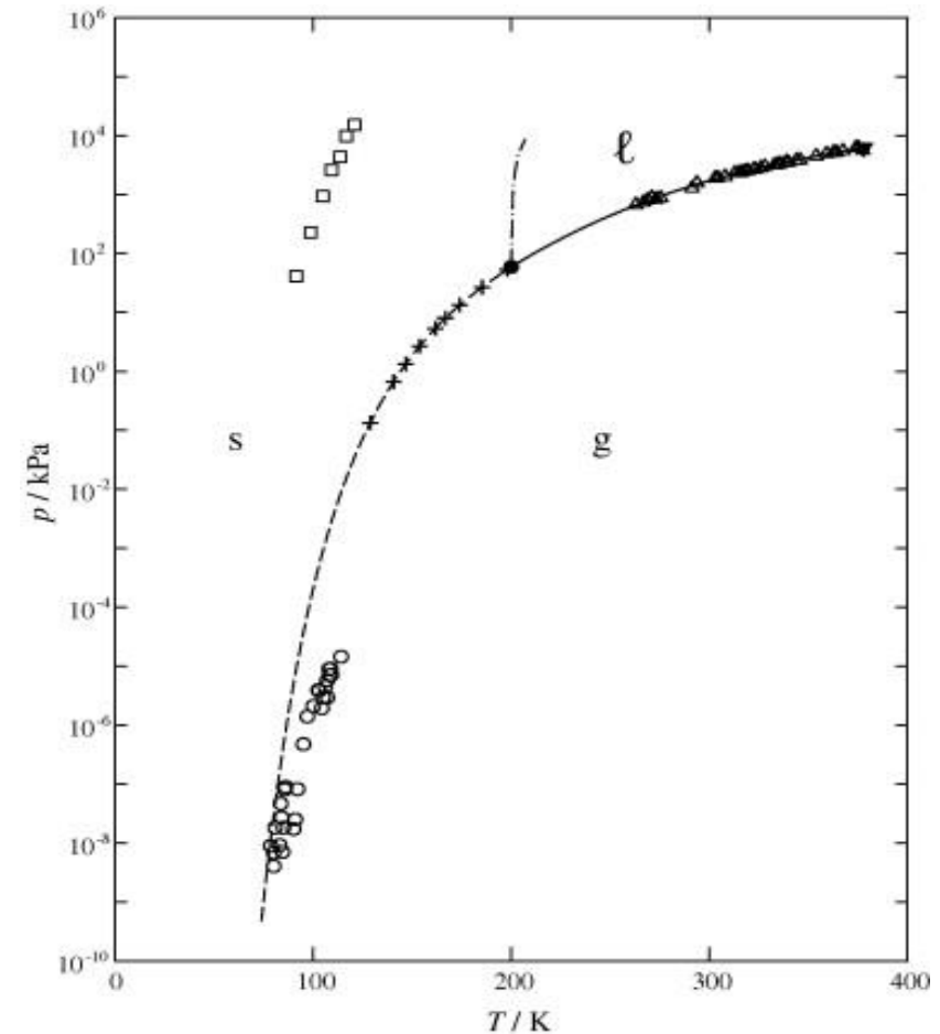
Phase diagram of radon, (A.G.M. Ferreira, 2007)
