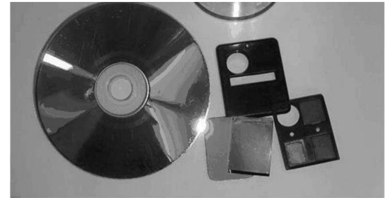
Based compact disc for retrospective radon measurement Dimitrova I., Pressyanov D., Georgiev S., Yankov P., Logistic of surveys of retrospective radon concentrations by home stored CDs/DVDs. Radiat. Prot. Dosim. 145, 300–304 (2011)
