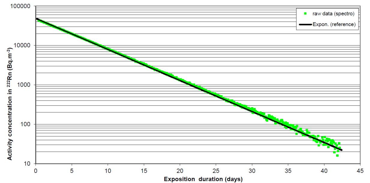
Lower background with spectrometry
