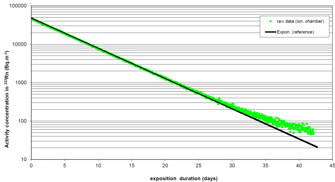
Impact of background with pulsed ion chamber
