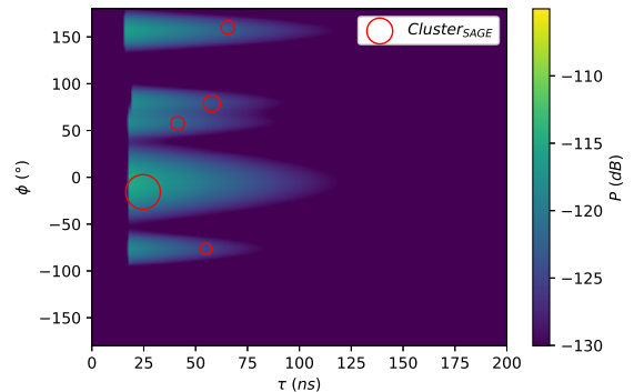
Fig. 8: Modeled DMCs PADP and SMCs cluster mean values LOS.
