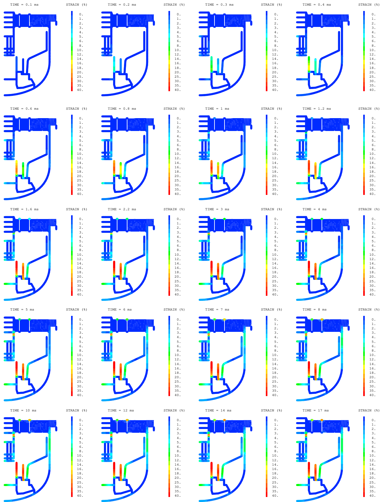
Fig. 13: Plastic strains
