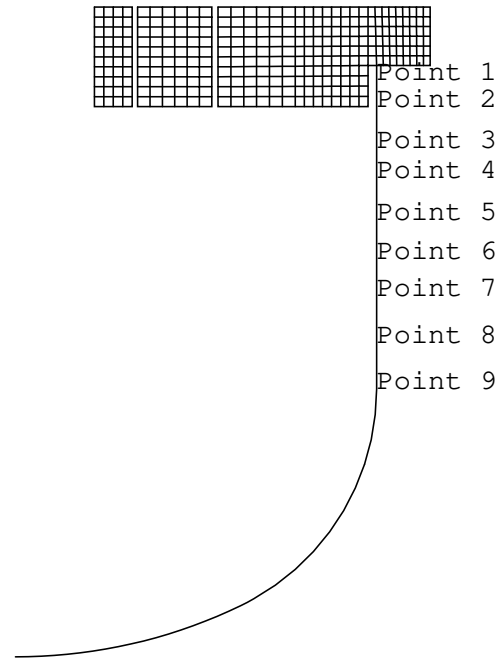
Fig. 8: Location of the points used to describe the main vessel upper bulge
