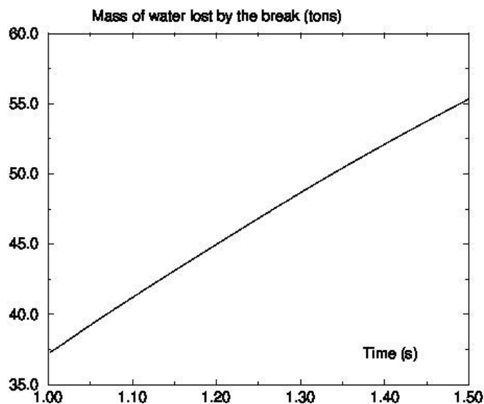
Figure 7 : Water mass loss at the break
