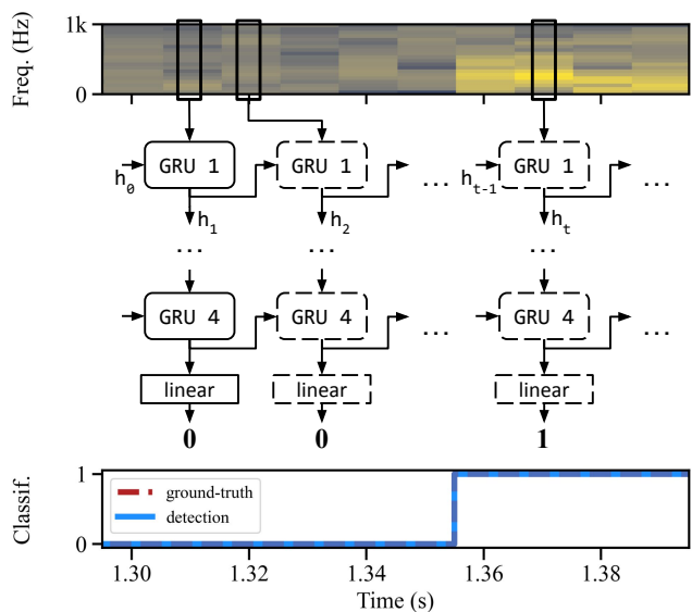
Fig. 4. Model architecture based on four stacked Gated Recurrent Units (GRU) classifying frequency-domain features to detect slip. The network processes the signal sequentially for a live scenario application, with 100Hz classification.
