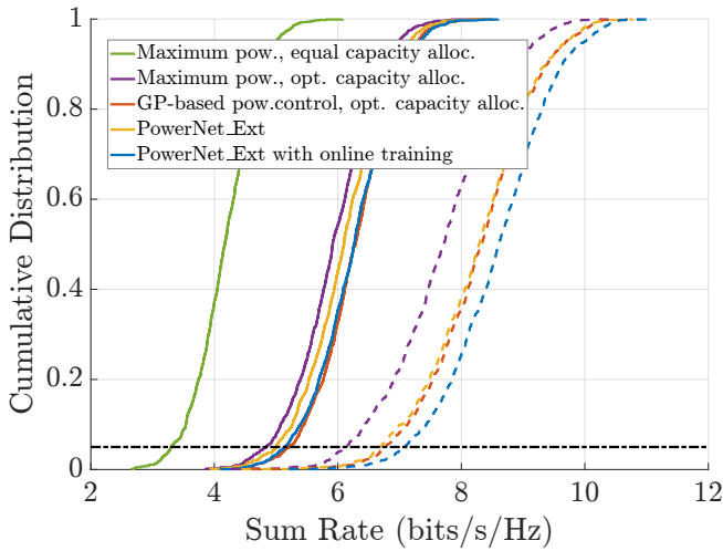
FIGURE 10. Sum rate comparison between PowerNet_Ext and the baseline [52] with joint power control and fronthaul capacity allocation for 50 APs and 10 users for ECF strategy. Total fronthaul capacity C_m = 1 bits/s/Hz. Solid lines: with transceiver hardware impairments ( \kappa_t = \kappa_r = 0.9 ) and dashed lines: perfect transceivers ( \kappa_t = \kappa_r = 1 ).
