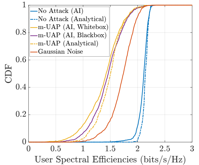
FIGURE 20. Comparison of different attack types ( \epsilon = 8 dB).
