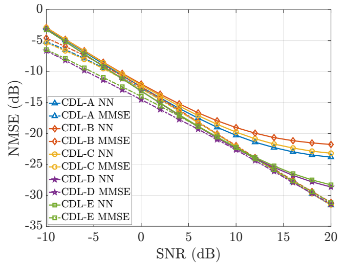
FIGURE 2. Our NN solution tested on different channel data produced from 3GPP CDL-A,B,C,D, and E channel models.
