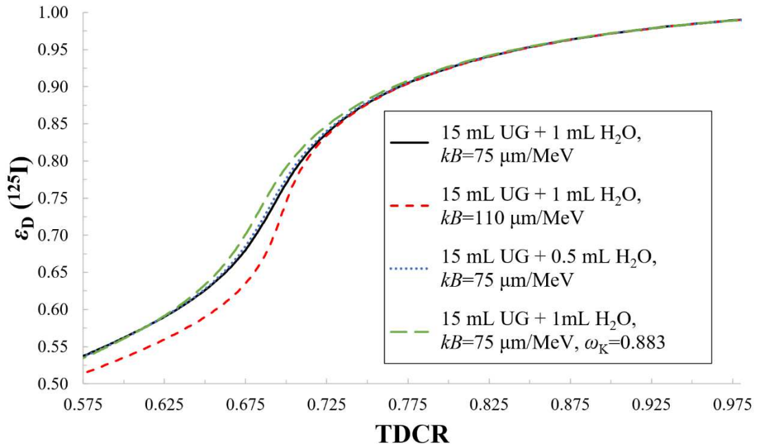
Figure 2: Computed efficiency \varepsilon_D for the logical sum of double coincidence as a function of the TDCR parameter. The black solid line was obtained for an LS composition with 15 mL UG and 1 mL \text{H}_2\text{O} and kB=75\text{ }\mu\text{m/MeV} while the red dashed line was obtained for the same composition but using kB=110\text{ }\mu\text{m/MeV} . The other curves were computed for an LS sample composition with 15 mL UG and 0.5 mL \text{H}_2\text{O} using \omega_K=0.875 (blue dotted curve) and \omega_K=0.883 (green long-dashed curve).
