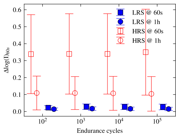
Figure 9 Impact of endurance cycling on current fluctuations. \Delta\log(I)_{60s} values at t=60s and t=1h for LRS and HRS after endurance cycling.
