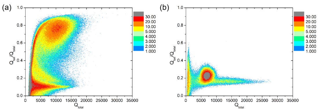
Figure 9. The 2-dimensional \alpha/\gamma PSD histograms of plastic scintillators (a) with 2 wt% CuI(PPh 3 ) 2 ( t -BuPy) and (b) with 2 wt% CuI(PPh 3 ) 2 ( t -BuPy) and 2 wt% PPO. Note that time gates and photomultiplier gain are not the same for both samples.
