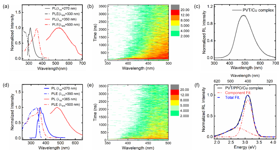
Figure 7. (a) PL and PLE spectra, (b) TRES and (c) X-ray excited RL spectrum of PVT/2 wt% CuI(PPh 3 ) 2 ( t -BuPy) plastic scintillator. (d) PL and PLE spectra, (e) TRES and (f) X-ray excited RL spectrum of PVT/2 wt% CuI(PPh 3 ) 2 ( t -BuPy)/2 wt% PPO plastic scintillator. The fitting curves are also shown.
