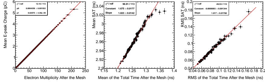
Figure 4: (left) The mean e-peak charge of simulated PICOSEC signals versus the respective “electron multiplicity after the mesh”. The middle and right plots demonstrate that the macroscopically determined PICOSEC SAT has the same properties as the microscopic variable “total-time after the mesh”, as it is described in the text.
