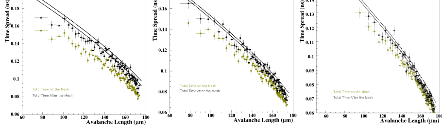
Figure 17: The points represent GARFIELD++ simulation results concerning the spread of the total time on the mesh (golden points) and the spread of the total time after the mesh (black points) versus the avalanche length. The solid lines represent predictions based on Eq. 63. The double lines indicate the systematic uncertainty due to the value of the w parameter, discussed in Section 6. The voltage settings considered in these comparisons are: 450 V at the anode and drift voltage of 325 V (left plot), 350 V (center plot), and 400 V (right plot).
