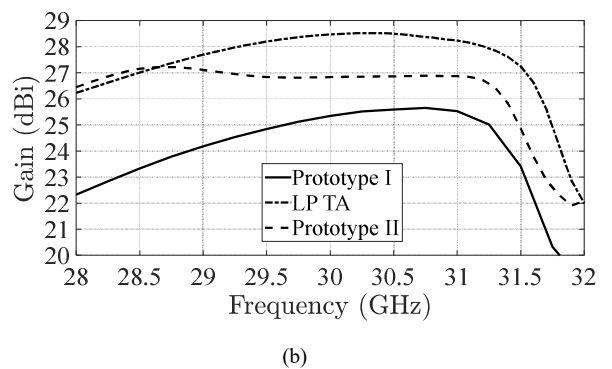
Fig. 5. Prototype II: (a) photograph. (b) Simulated peak gain, including comparison with the performance achieved with the prototype I and the 2-bit linearly-polarized transmitarray.
