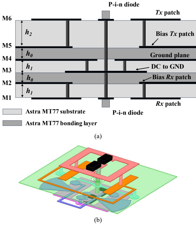
Fig. 1. 2-bit linearly-polarized unit-cell with p-i-n diodes. (a) Dielectric stack-up and (b) 3D view
