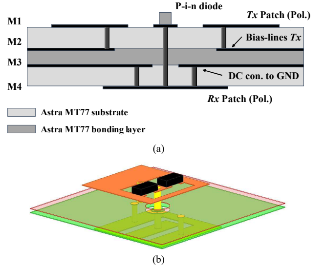
Fig. 2. Linear to circular polarization converter with p-i-n diodes. (a) Dielectric stack-up and (b) 3D view.
