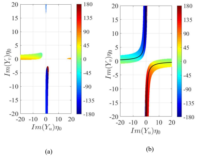
Fig. 2. Phase of transmission, T_{yx} , as a function of the rotator normalized admittance that describes its properties in the crystal system (uv) . The polarizers are assumed ideal; the spacers have a permittivity \epsilon_r = 3 and thicknesses equal to (a) h_1 = 0.25\lambda , h_2 = 0.125\lambda and (b) h_1 = h_2 = 0.25\lambda . Both graphs depict only the part of the phase where the reflection loss is less than 1 dB. The solid curve in (b) represents the solutions of the admittance pairs (Y_u, Y_v) where there is perfect transmission.
