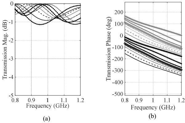
Fig. 7. Magnitude (a) and phase (b) of T_{xx} for the designed quartz UC. The mirrored cases in the phase of transmission are depicted in grey color. All UC use the same rotator topology (Fig. 6b); the transmission phase is tuned by varying their angle \varphi_g from 20^\circ to 50^\circ and the angle \varphi_{off} from 0^\circ to 40^\circ .
