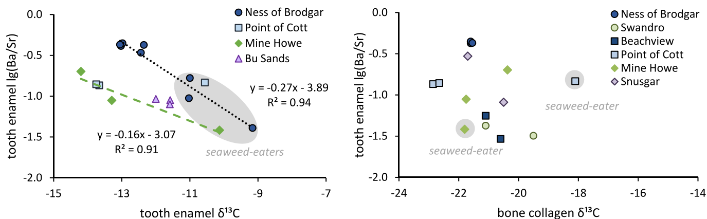
Fig. 4. Archaeological sheep tooth enamel \lg(\text{Ba}/\text{Sr}) plotted against \delta^{13}\text{C} data (shown here without adjusting for the fossil fuel effect) of enamel shown on the left, and mandible bone collagen \delta^{13}\text{C} on the right. The linear trendlines are for data from Mine Howe (dashed), and Ness of Brodgar (dotted). The shaded areas indicate sheep interpreted to have been consuming seaweed (particularly in winter) based on sequential enamel \delta^{13}\text{C} and \delta^{18}\text{O} results from the same teeth (Balasse et al., 2009 and Blanz et al. forthcoming); such data was unavailable for sheep from Bu Sands, Swandro, Beachview and Snusgar.
