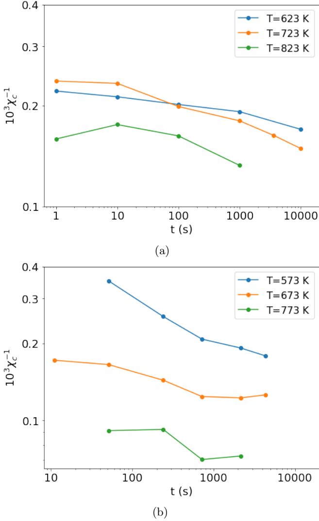
Figure 8: Evolution of the inverse susceptibility with annealing time at different annealing temperatures: (a) IF steel, (b) ELC steel.
