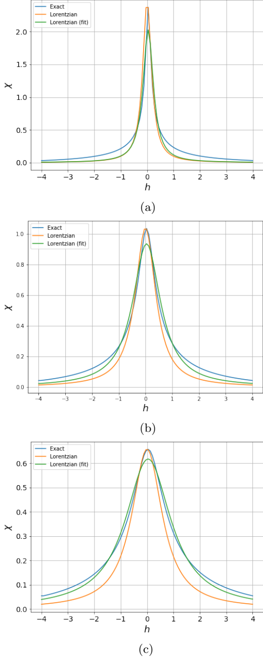
Figure 2: Comparison of the exact solution (10) ("Exact") with the expression (18) ("Lorentzian") and a fitted Lorentzian ("Lorentzian fit") for three different disorder values. (a) r = 5.11 , (b) r = 5.55 and (c) r = 6.0 .
