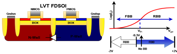
Figure 1: Cross-section of LVT FDSOI transistor.
