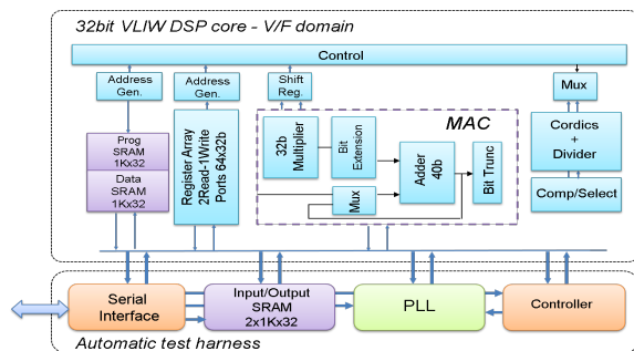
Figure 2: Block diagram of 32-bit DSP.
