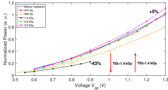
Figure 7: Power degradation at different TID levels.
