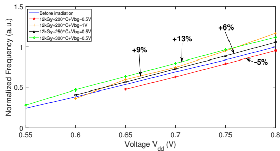
Figure 9: Frequency recovery after applying the T- V_{bg} method.
