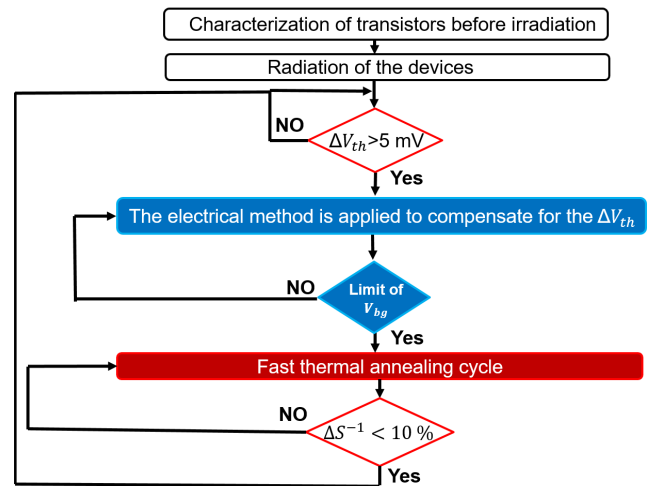
Figure 8: Flow diagram of the mixed hardening methodology.
