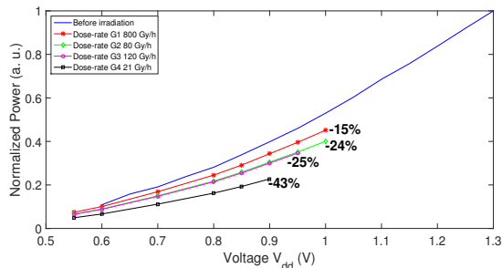
Figure 12: Power degradation at different dose-rates.
