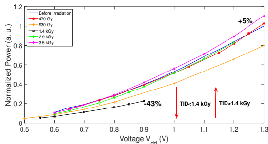
Figure 7: Power degradation at different TID levels.
