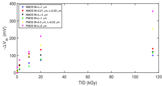
Figure 5: Threshold voltage degradation for 28nm FDSOI-LVT single transistors.
