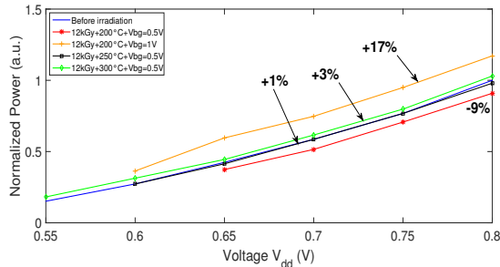
Figure 10: Power recovery after applying the T- V_{bg} method.
