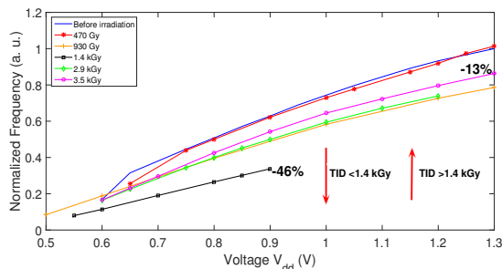
Figure 6: Frequency degradation at different TID levels.
