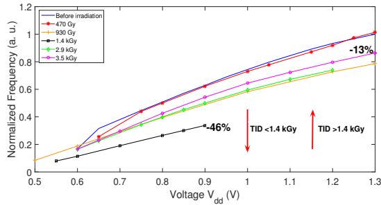
Figure 6: Frequency degradation at different TID levels.
