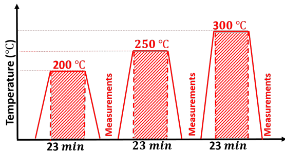
Figure 3: Annealing procedure.
