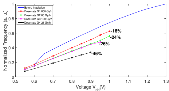
Figure 11: Frequency degradation at different dose-rates.
