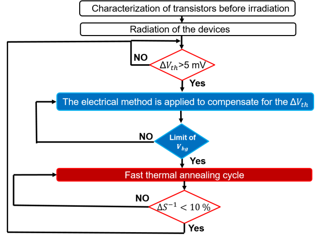
Figure 8: Flow diagram of the mixed hardening methodology.
