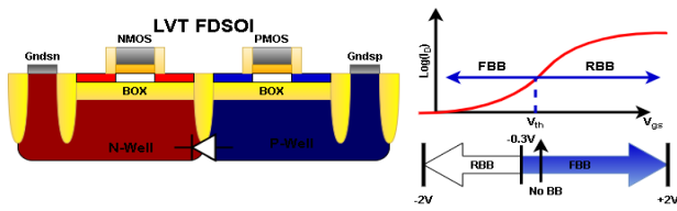
Figure 1: Cross-section of LVT FDSOI transistor.
