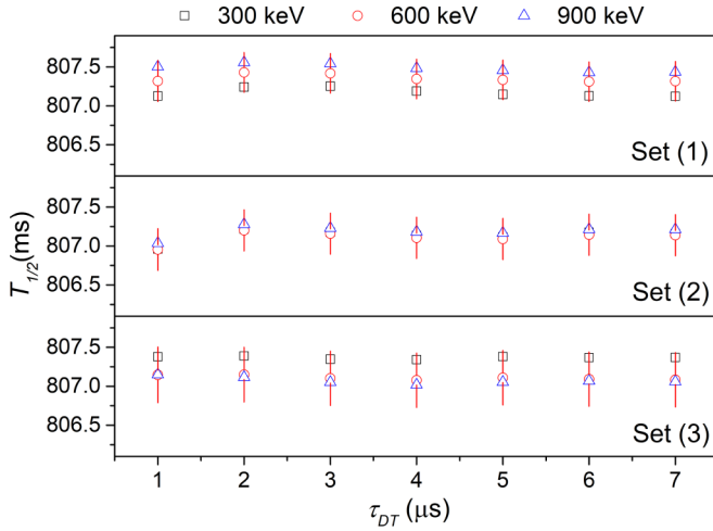
FIG. 11. Mean values of the half-life estimates obtained for set 1 (top), 2 (middle), and 3 (bottom) as a function of the nonextendable dead time. The black squares, red dots, and blue triangles correspond respectively to offline energy thresholds of 300, 600, and 900 keV. The statistical error bars are only shown for the threshold of 600 keV.
